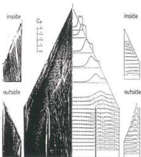
Fig. 12: Pressure distribution and surface oilflow pattern on the wing-fin configuration SH at \alpha = 20^\circ , \beta = 0^\circ (Oilflow patterns from the fin enlarged).
