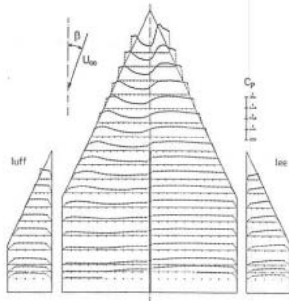
Fig. 11: Pressure distribution on the wing-fin configuration MC at \alpha = 25^\circ , \beta = 20^\circ .
