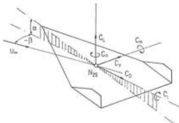
Fig. 4: Experimental coordinate system for windtunnel data reduction.
