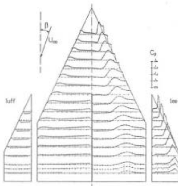
Fig. 8: Pressure distribution on the wing-fin configuration MC at \alpha = 10^\circ , \beta = 20^\circ .
