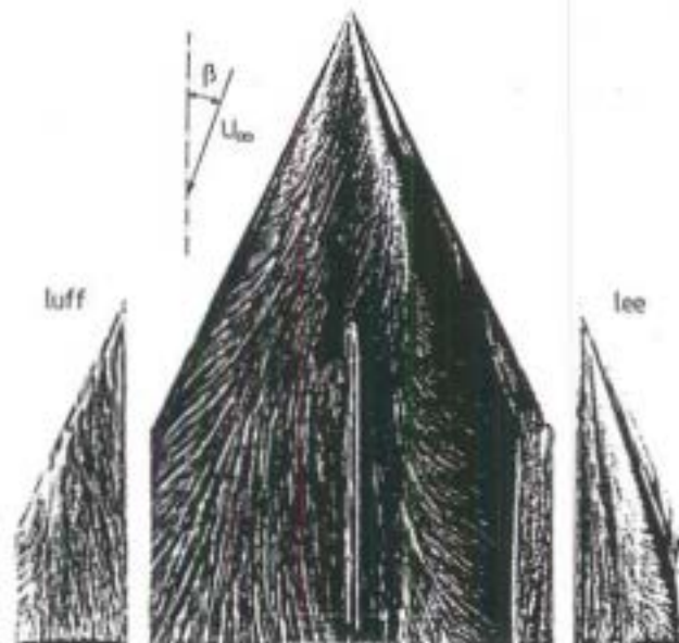
Fig. 9: Surface oilflow pattern on the wing-fin configuration MC at \alpha = 10^\circ , \beta = 20^\circ .
