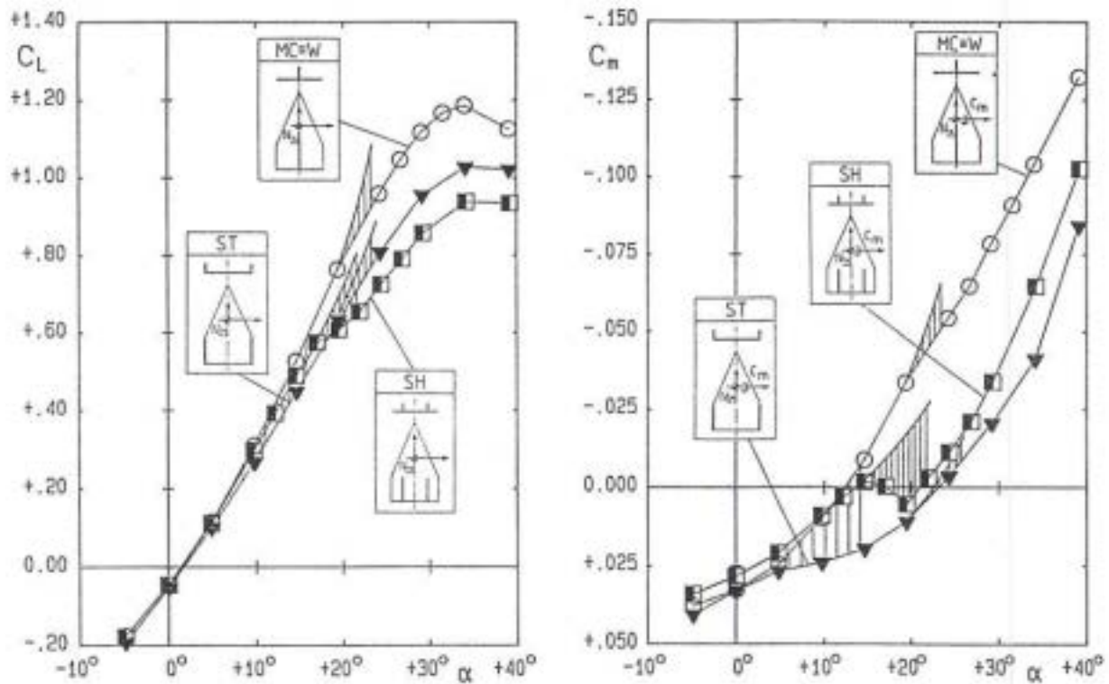
Fig. 5: Lift and pitching moment characteristics for the wing alone W and the wing-fin configurations MC, SH, ST in symmetrical flow.
