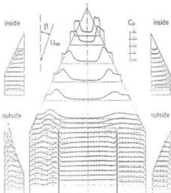
Fig. 13: Pressure distribution on the wing-fin configuration SH at \alpha = 20^\circ , \beta = 5^\circ .
