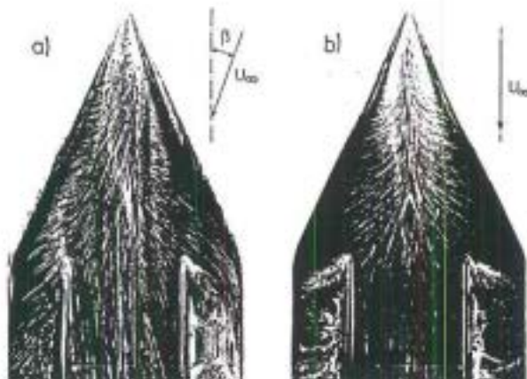
Fig. 14: Surface oilflow pattern on the wing of the wing-fin configuration SH at a) \alpha = 20^\circ , \beta = 10^\circ and b) \alpha = 30^\circ , \beta = 0^\circ .
