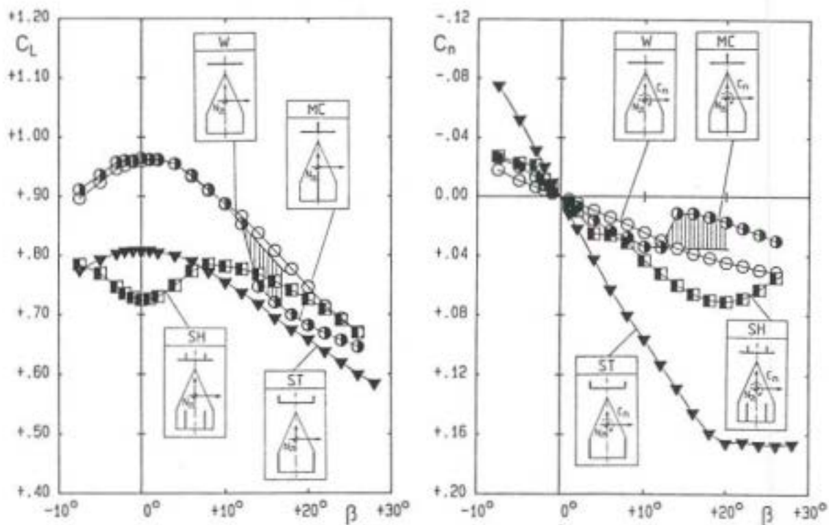
Fig. 7: Lift and yawing moment characteristics for the wing alone W and the wing-fin configurations at \alpha = 25^\circ .
