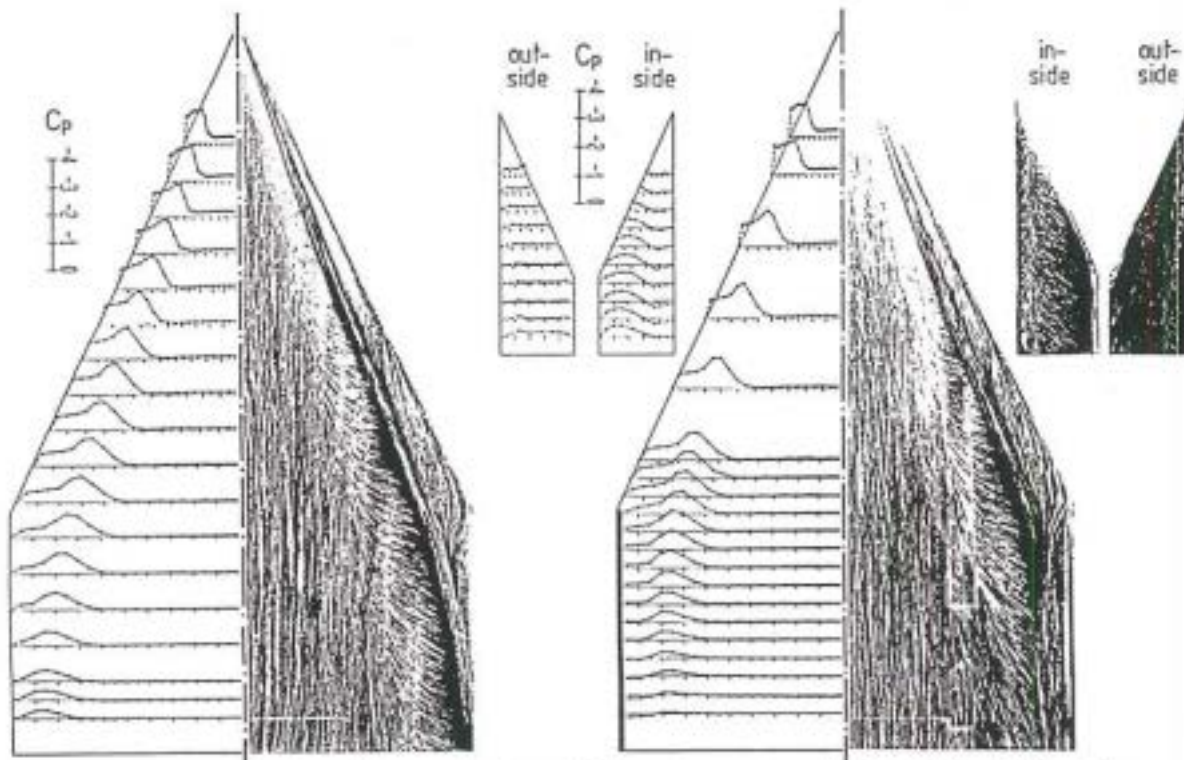
Fig. 15: Pressure distribution and surface oilflow pattern at \alpha = 10^\circ , \beta = 0^\circ for a) Wing alone (W) and b) Wing-fin configuration ST (Oilflow patterns from the fin enlarged).
