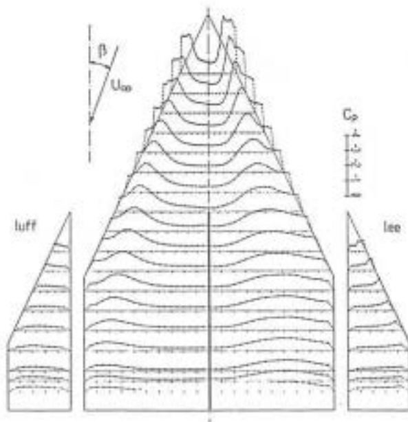
Fig. 10: Pressure distribution on the wing-fin configuration MC at \alpha = 25^\circ , \beta = 10^\circ .
