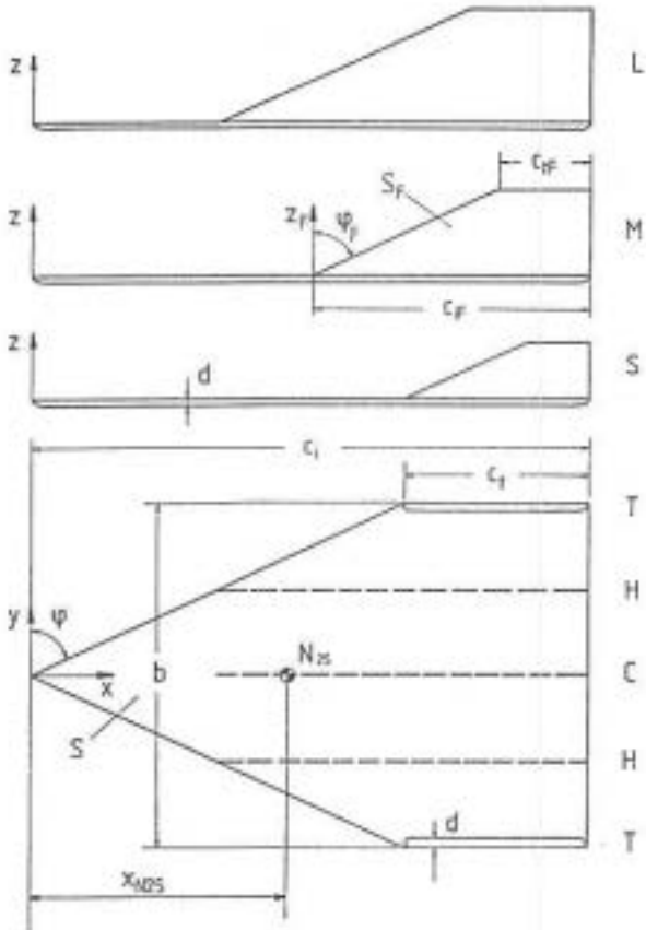
Fig. 1: Cropped delta wing ( A = b^2/S = 0.93 , \lambda = c_t/c_i = 1/3 , \varphi = 65^\circ , flat plate) with half-wing-shaped vertical fins of different size (S, small, c_{iF}/c_i = 1/3 ; M, medium, c_{iF}/c_i = 1/2 ; L, large, c_{iF}/c_i = 2/3 ) in various spanwise positions (C, central; H, half semispan; T, tip).
