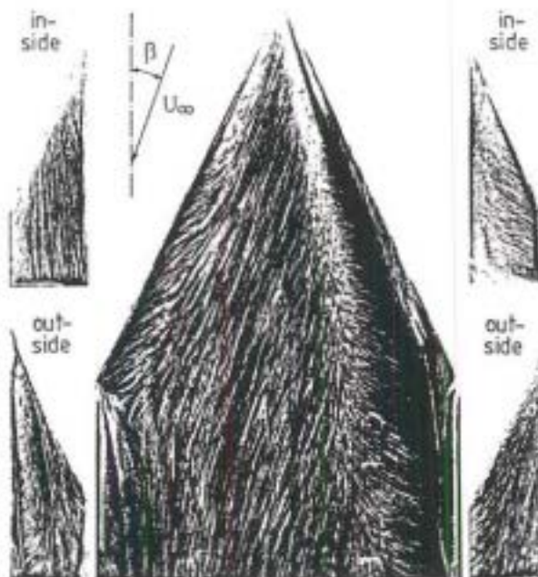
Fig. 17: Surface oilflow pattern on the wing-fin configuration ST at \alpha = 10^\circ , \beta = 20^\circ (Oilflow patterns from the fins enlarged).
