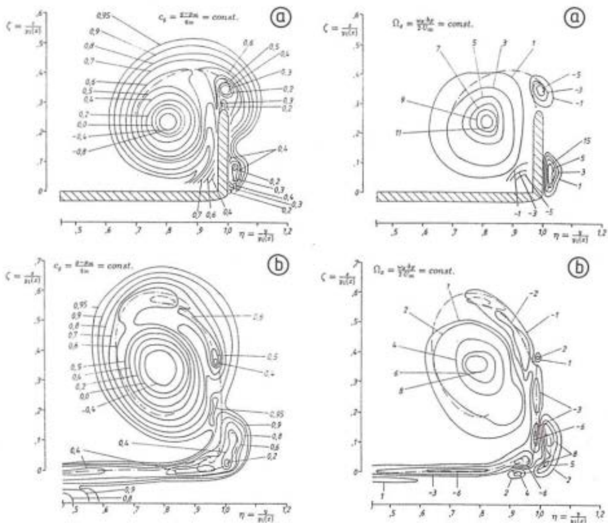
Fig. 18: Flowfield on the wing-fin configuration ST at \alpha = 13.5^\circ , \beta = 0^\circ in cross-sections at a) \xi = 0.85 and b) \xi = 1.01 . Lines of constant total pressure lefthand and lines of constant axial vorticity righthand.
